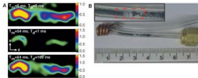
(A) MRI images show polarised propane moving through the catalyst, revealing whether further reaction takes place. (B) Catalytic reactor with Wilkinson's catalyst powder mixed with glass beads. An enlarged view of the catalyst packing is shown in the inset. The dashed red lines indicate the field of view for the images
