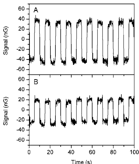
FIG. 8. Sensitivity comparison between the gradiometer and the primary channel. The test signal is a 40 nG magnetic field modulated at 0.1 Hz, produced by the z -gradient coil which is powered by a function generator. Plot A shows the gradiometer signal with closed feedback loop on the primary-channel magnetometer. Plot B shows the signal from the primary-channel magnetometer with the feedback loop open.
